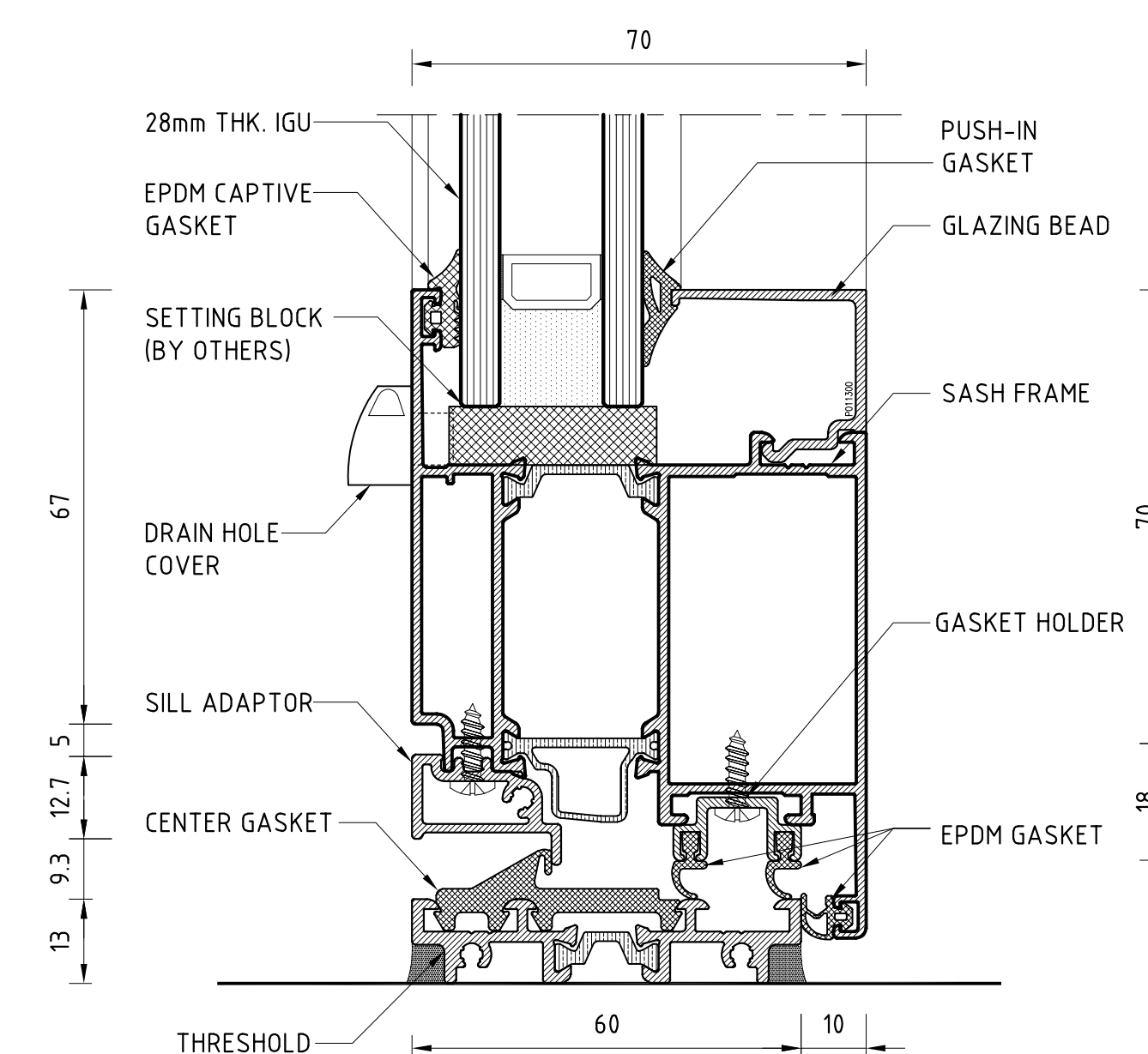
SILL DETAIL
